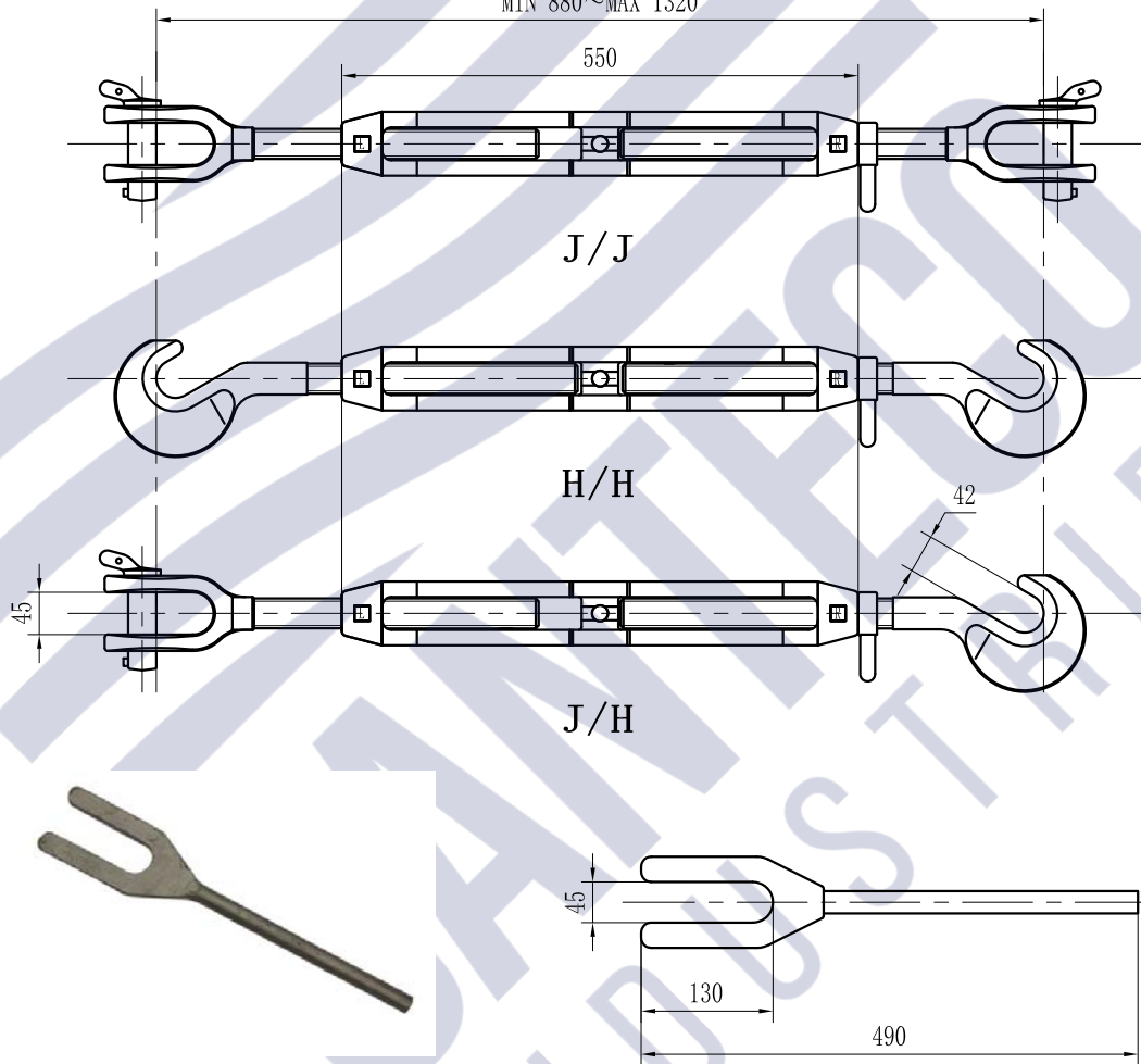
Turnbuckles Spanner
